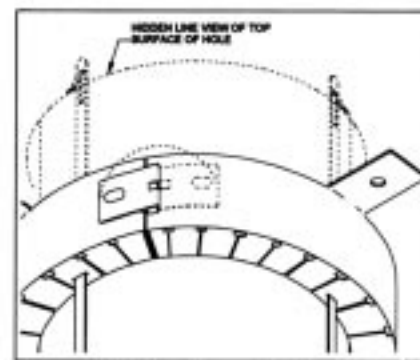
Figure 2: PPD positioned and anchor straps inserted
