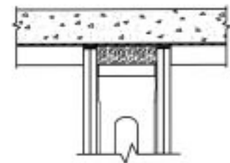
3M FireDam 150+ Caulk used in applications with dynamic head-of-wall joints where gypsum wall board is sculptured into the fluted deck. UL System H-WD-0111.
