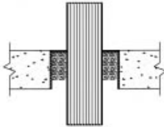
3M FireDam 150+ Caulk used in applications where cable bundles penetrate through concrete. UL System C-AJ-3 I 64.
