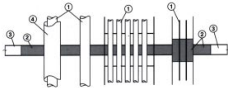
1. Penetrations 2. Filler Material 3. Floor or Wall 4. Pipe Insulations
