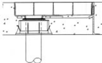
Install pipe - complete assembly
